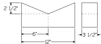
WOOD BUNK FOR 4-TBR80
